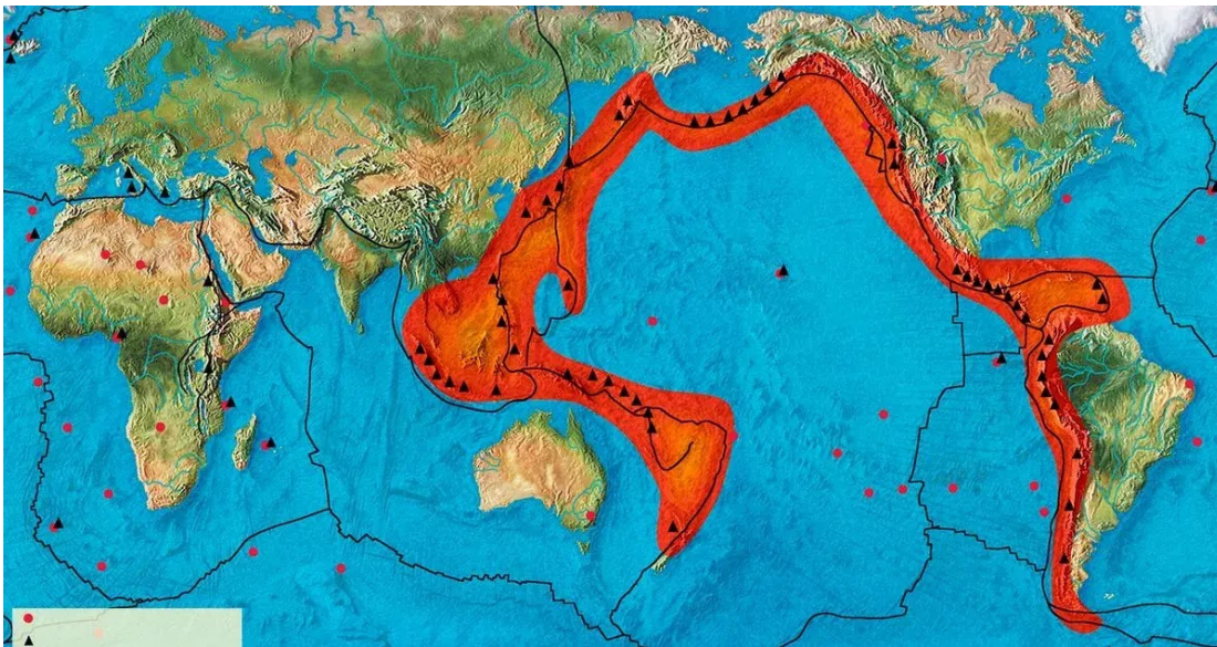
Ring of Fire
