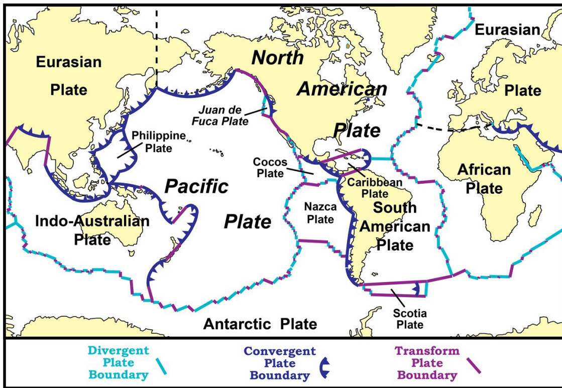
Seven Major Crustal Plates
